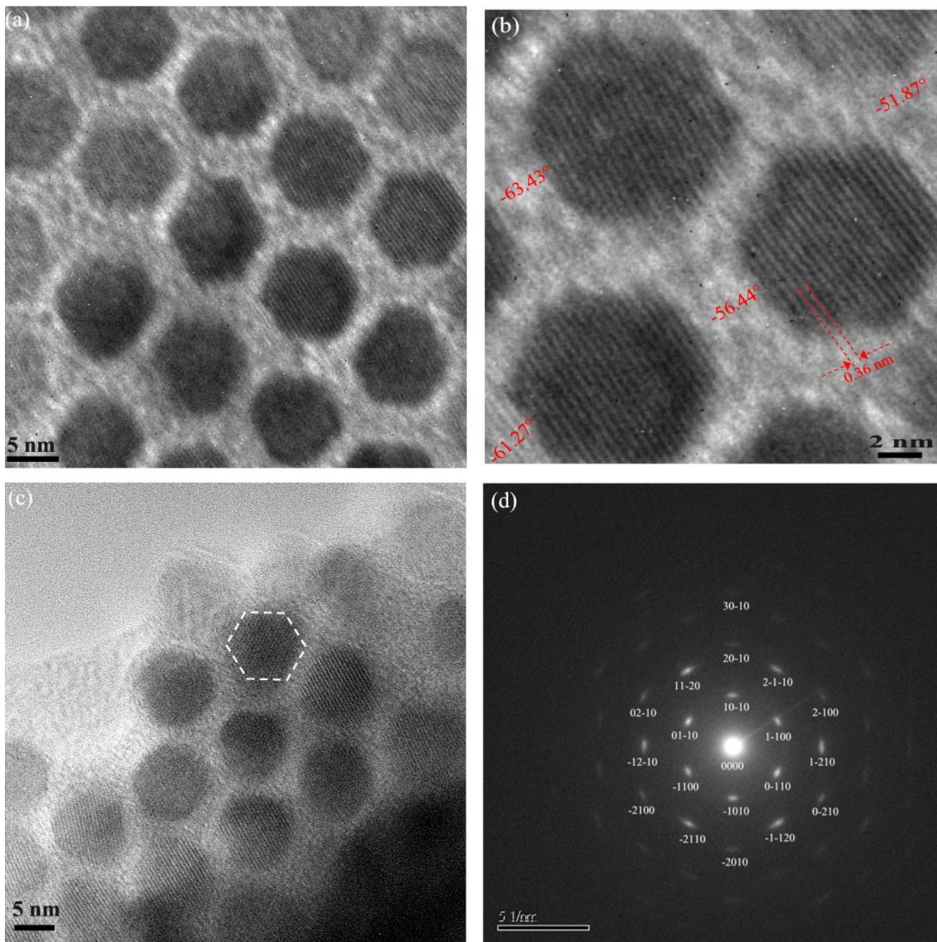
Figure 5. High resolution TEM images, acquired from the same domain as shown in figure 3 showing atomic lattice fringes and electron diffraction: (a) TEM image, acquired from the centre of figure 3a, shows lattice fringes from (100) planes of wurtzite CdS rods (scale bar = 5 nm). (b) Further magnified HRTEM image (scale bar = 2 nm) with an angular variation in lattice fringing of \pm 6^\circ . Highlighted lattice spacing of 0.36 nm is consistent with (100) planes of wurtzite CdS. (c) HRTEM image acquired from the edge of the domain shows large variation in angular rotation of the lattice fringes. (d) Single crystal electron diffraction indexing of CdS nanorods in the [0001] beam direction.
