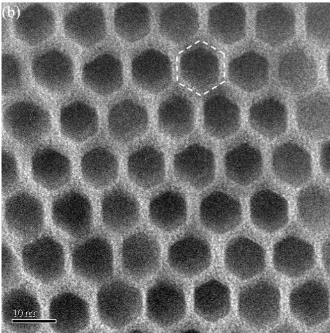
Figure 3. TEM images of perpendicularly aligned nanorod superlattice: (a) TEM image acquired from the centre of a domain (scale bar = 50 nm). Highlighted region A and B show repeating hexagonal geometry and nanorod vacancy respectively (b) Further magnified TEM image (scale bar = 10 nm), highlighted region shows perfect faceting of the wurtzite nanorod.
