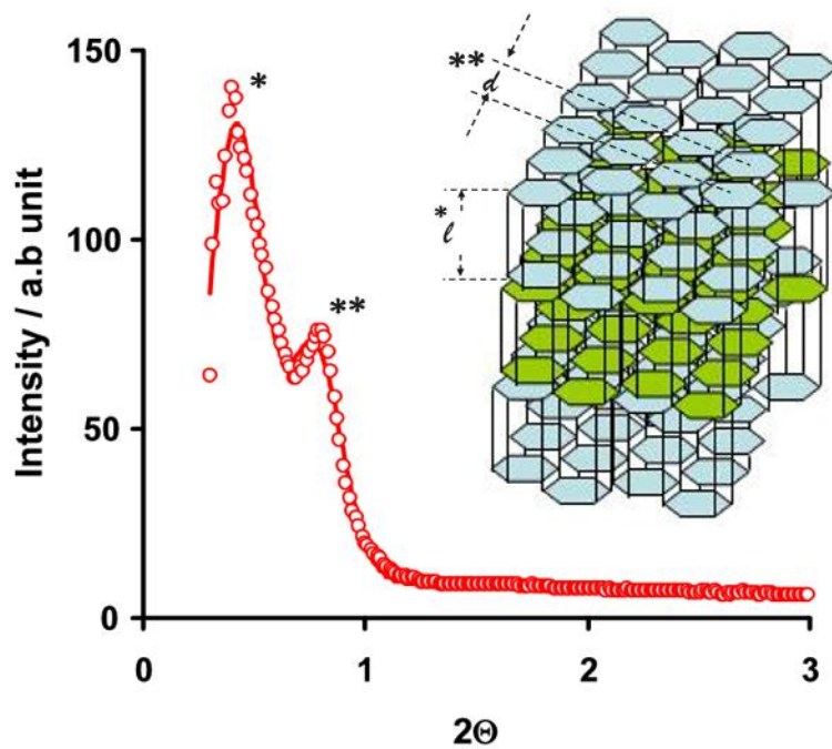
Figure 4. Plot of intensity (arbitrary unit) vs. 2\Theta (degree) from small angle x-ray scattering (SAXS) data (curve fitted with correlation value R^2 = 0.994 ). Two reflections are indexed at 2\Theta = 0.417 and 0.770 respectively corresponding to diffraction from lattice repetition along the nanorods length, l and across nanorod rows, d as shown in the inset schematic.
