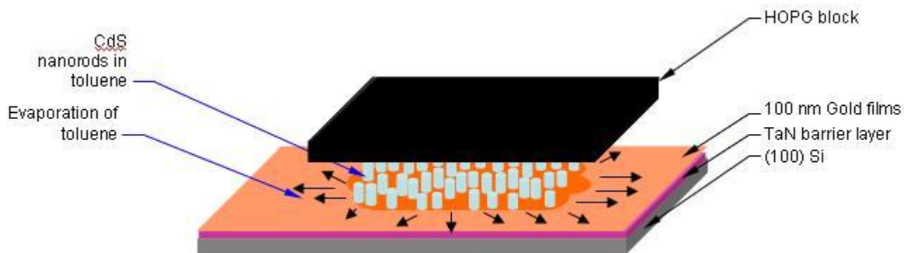
Figure 1. The 3D schematic shows the set-up used for monolayer nanorod assembly. A nanorod toluene solution was trapped between the gold sputtered substrate ( Si / TaN /Au, 0.5 mm / 40 nm / 100 nm) and a highly ordered pyrolytic graphite block (HOPG, 20 mm × 20 mm × 1 mm, SPI Supplies) and allowed to dry over several hours under controlled evaporation conditions.
