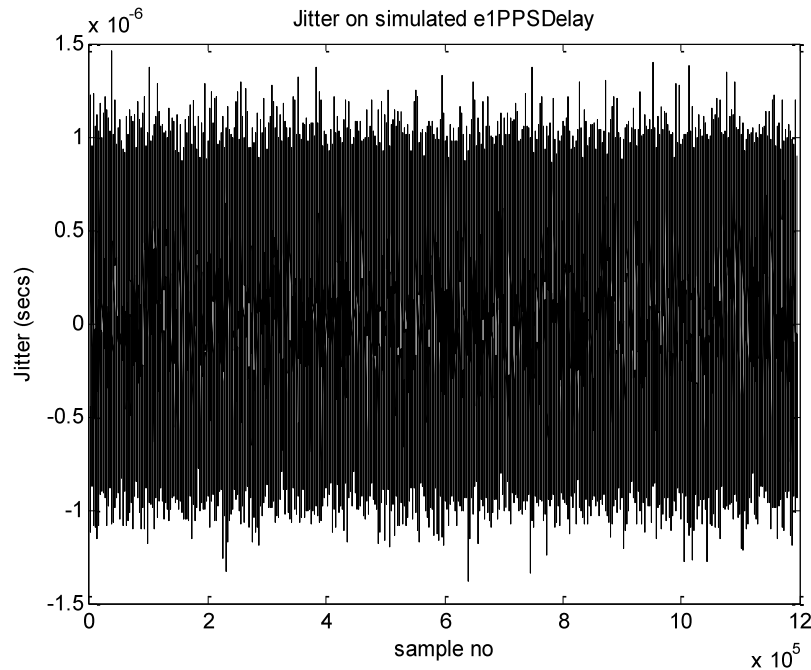
Figure 10. Simulation version 1: Jitter on simulated e1PPSDelay at slave station.
