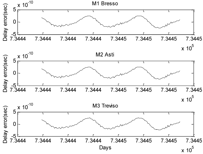
Figure 12. Delay error due to simulated satellite motion in 3-station simulation.
