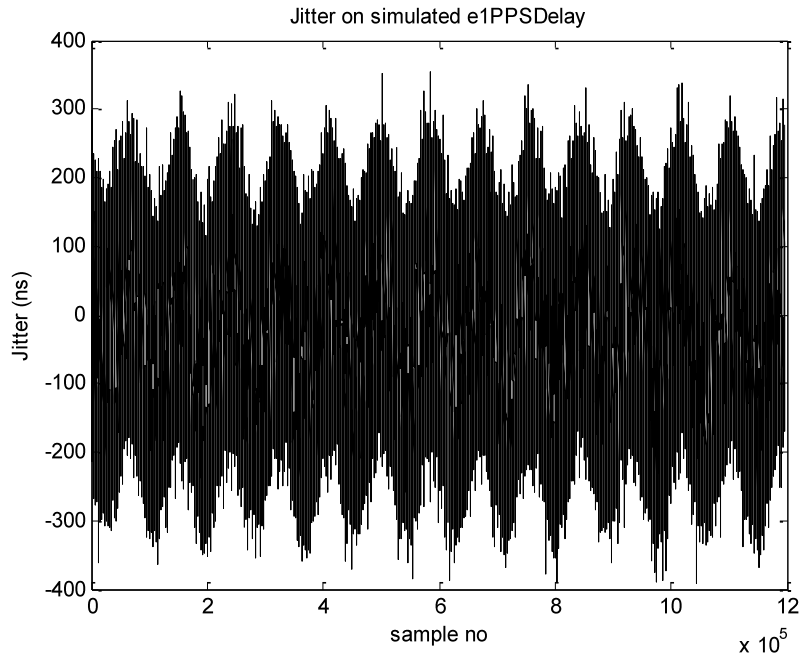
Figure 11. Simulation version 2: Jitter on simulated e1PPSDelay at slave.
