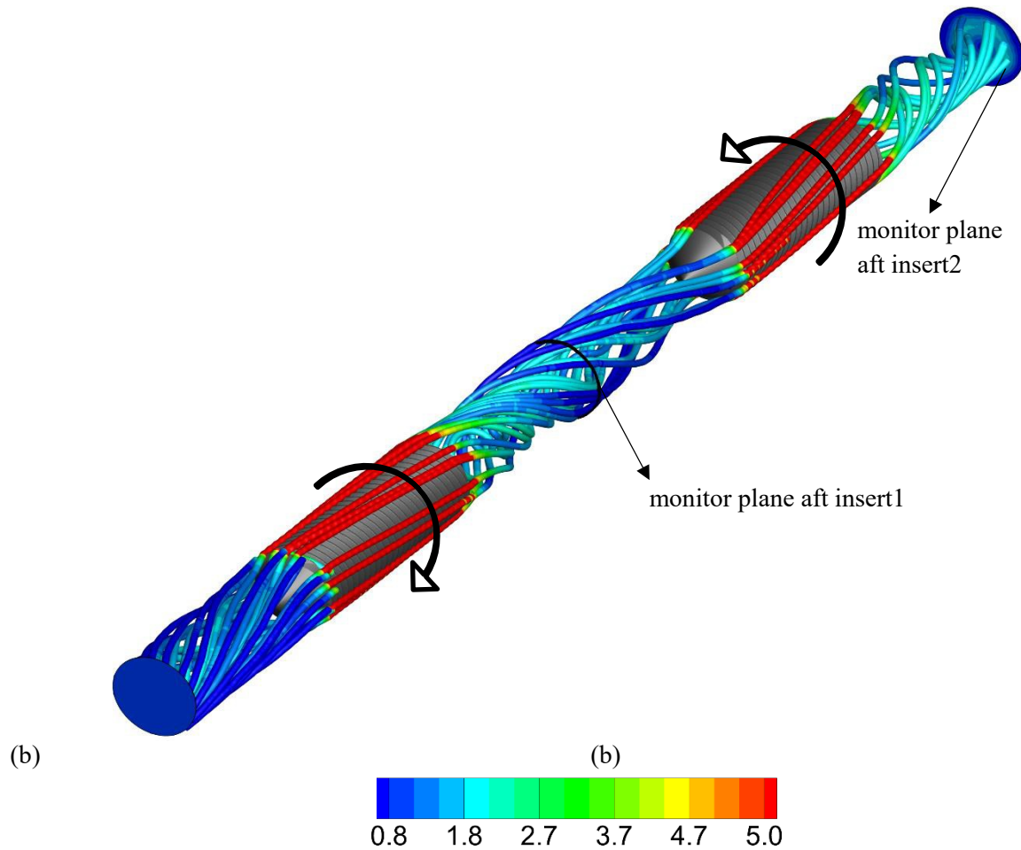
Figure 3: Stream traces coloured by non – dimensional velocity magnitude using inlet velocity over 5-channel inserts at Re = 400 . (a) Cross-flow effect between the stream traces; (b) Switching of flow direction aft inserts
