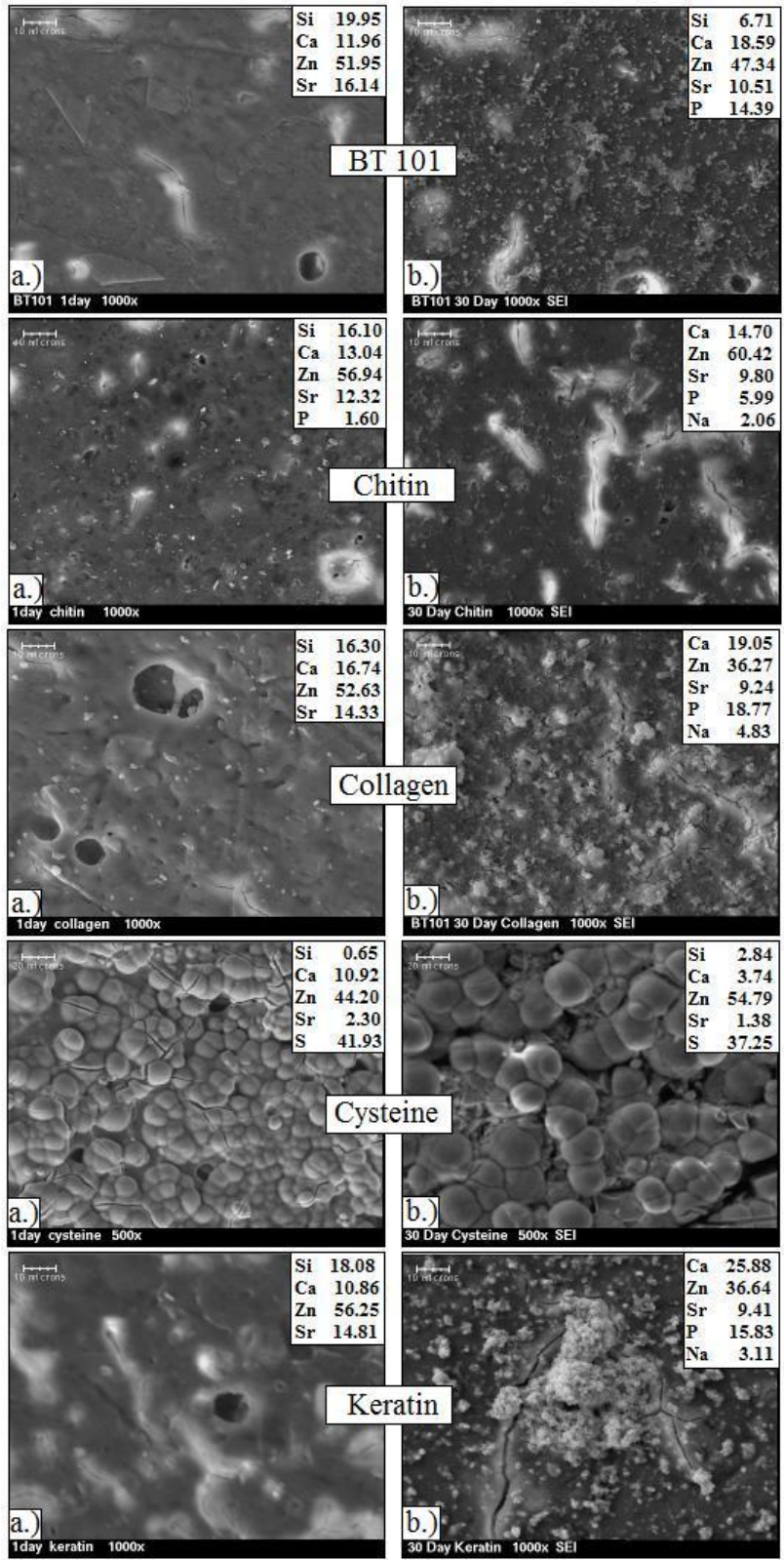
Figure 5. SBF results of modified cement series after a.) 1day and b.) 30 days.
