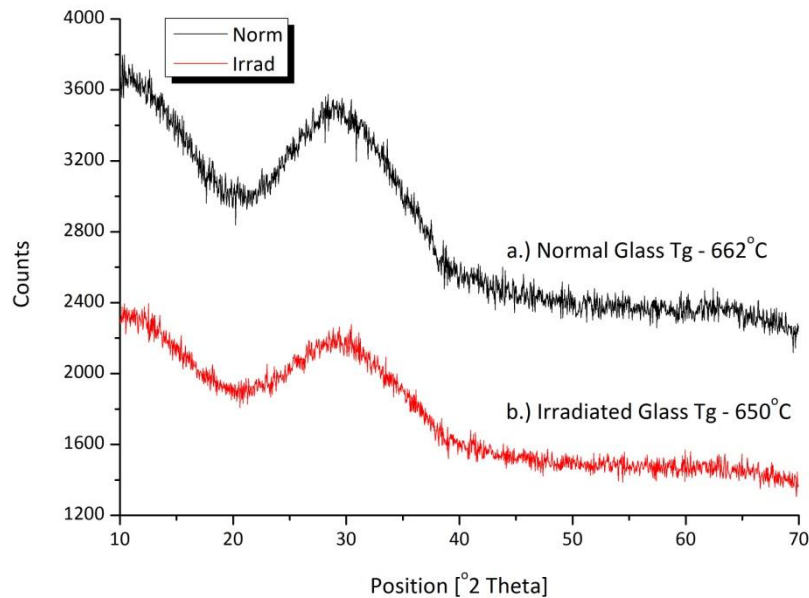
Figure 1. Characterization of glass used for cement series.
