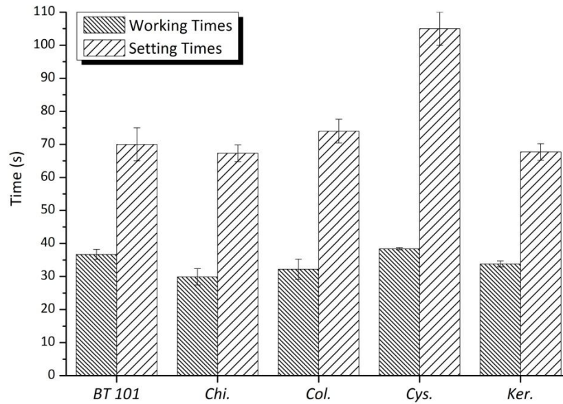
Figure 2. Working and setting times of cement series.
