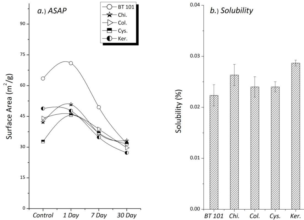
Figure 4. Surface area and solubility of cement series as determined by ASAP.
