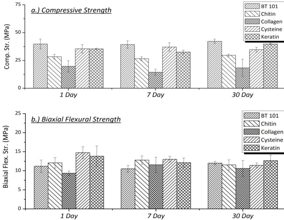
Figure 3. a.) Compressive strength and b.) Biaxial flexural strength of modified cement series.
