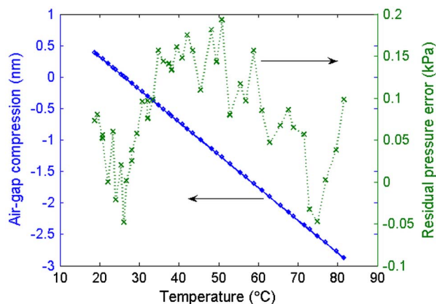
Fig. 4. Temperature sensitivity of the EFPI probe. The chart reports the air-gap compression as a function of temperature (left axis), with an estimated slope 51.9 \text{pm}/^\circ\text{C} , and residual error after temperature compensation (right axis).
