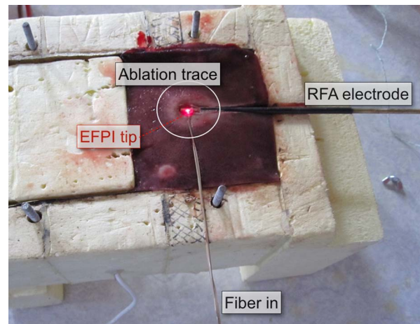
Fig. 12. Setup for third ex vivo RFA experiment: porcine liver has been inserted in a small chamber to facilitate positioning. Electrode and optical fiber probe are inserted perpendicularly, with a 0.5 cm misalignment between the two tips, only a few millimeters below the liver tissue. The picture, taken after the ablation, shows elliptical shape traces with the thermal lesion (light colored tissue). The optical fiber tip is illuminated with a red laser, and is located in close proximity of the center of the ablation lesion; the illumination shows the 0.5 cm misalignment between the electrode tip and the fiber output.
