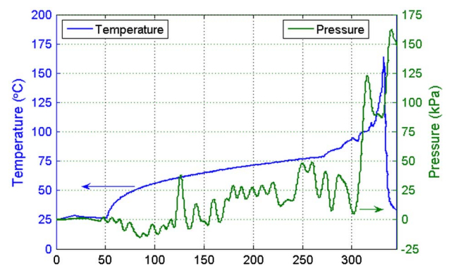
Fig. 10. Second RFA experiment: temperature and pressure traces; x axis shows time, in s.
