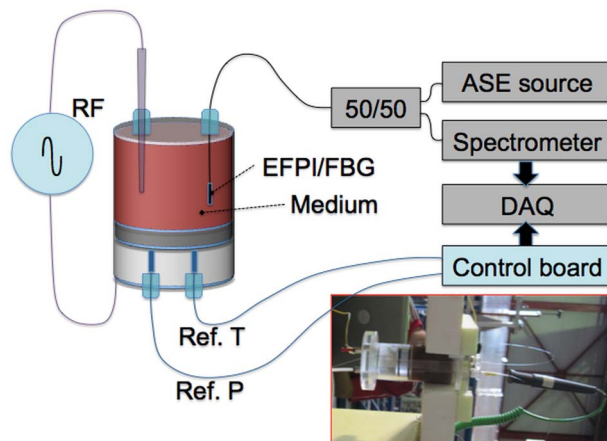
Fig. 5. RF-heated test chamber setup. The inset shows a picture of the setup, loaded with liver on the top chamber.
