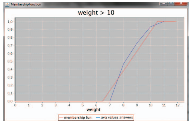
(b) Generated membership function
