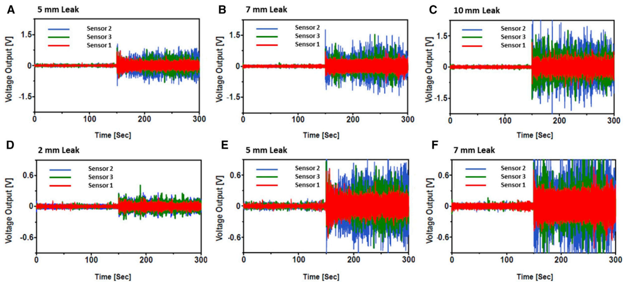
Figure 6. Amplitude-based analysis to determine leak location
