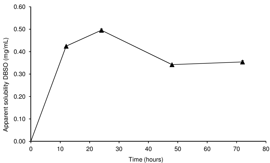
Figure 7: Dynamic solubility profile of DBSO from cocrystal in presence of 6 mg/mL BA over 72 hours.
