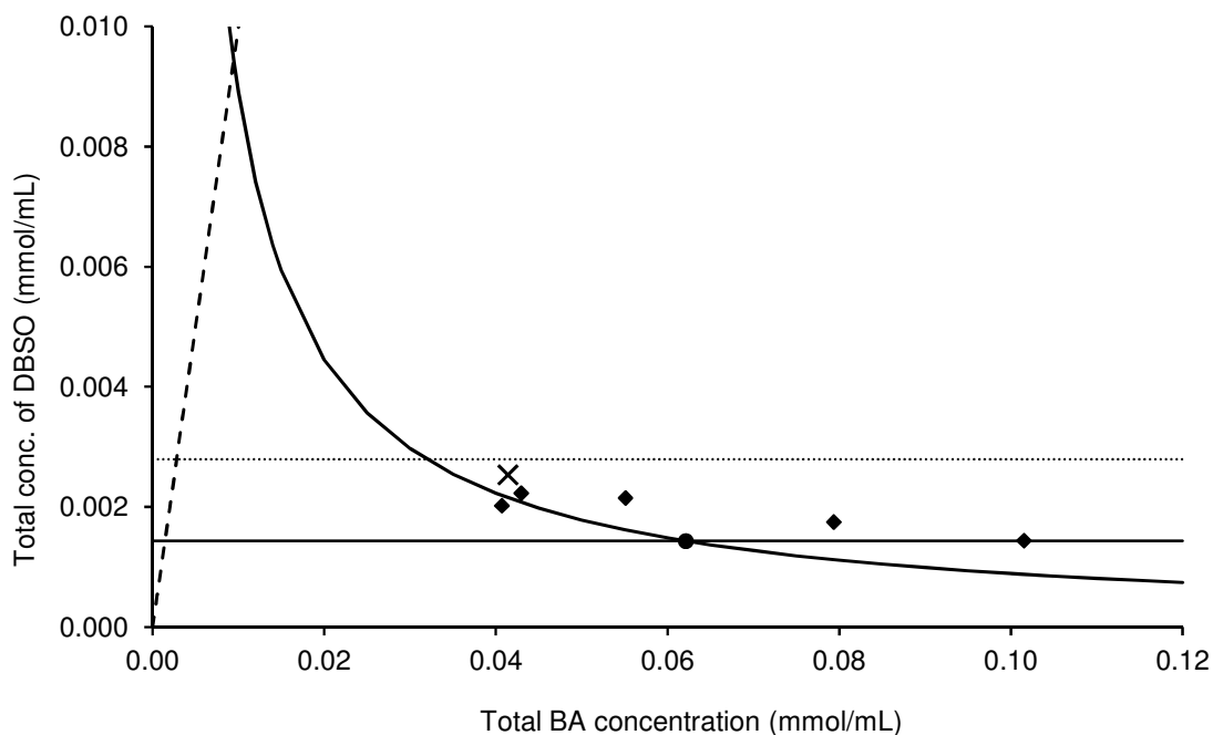
Figure 8: Phase solubility diagram of 1:1 BA:DBSO cocrystal. The horizontal line marks the solubility of pure DBSO, the curved line represents the cocrystal solubility curve determined by equation 3, the dotted line represents the solubility limit of complex as determined from the plot presented in Figure 4, the filled diamonds mark the experimental cocrystal solubility values (BA dependent), the dashed line represents stoichiometric concentrations of cocrystal components that dissolution could follow in ideal case, the filled circle symbolizes the transition concentration (DBSO/CC) and the cross illustrates the experimental obtained transition concentration (DBSO/CC).
