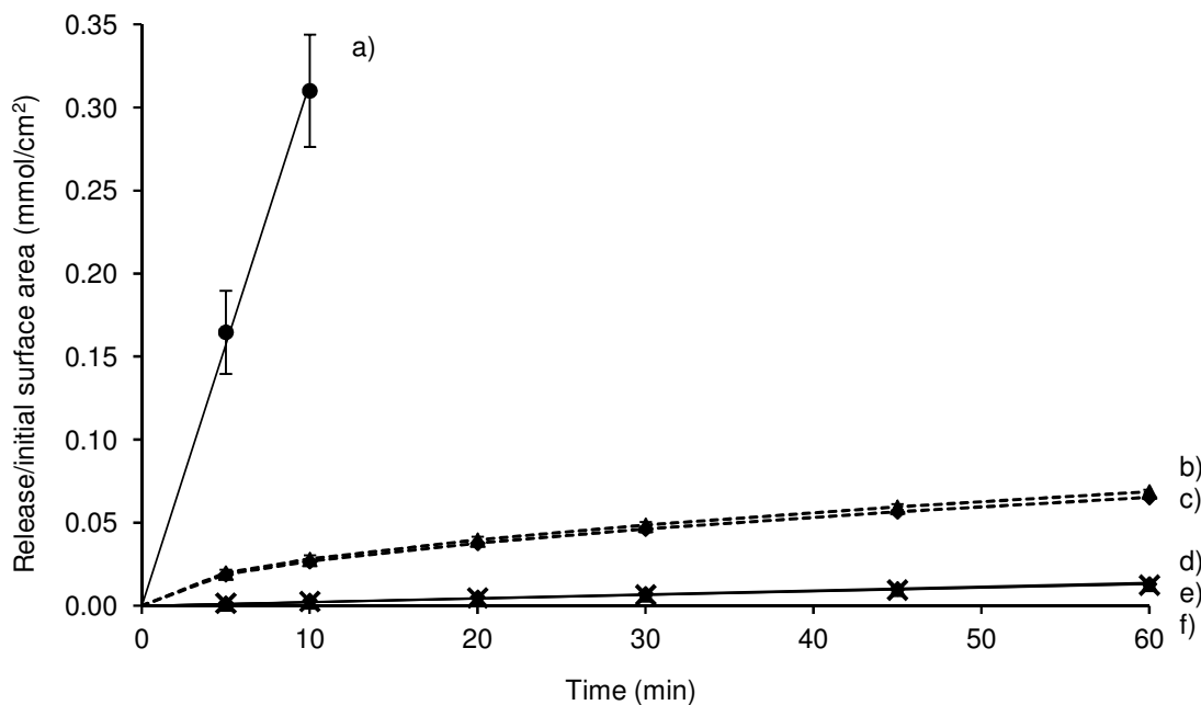
Figure 11: Dissolution profiles of (a) BA, (b) BA from a physical mixture, (c) BA from the cocrystal, (d) DBSO from a physical mixture, (e) DBSO from the cocrystal and (f) DBSO. The dashed line refers to the square-root of time fit.
