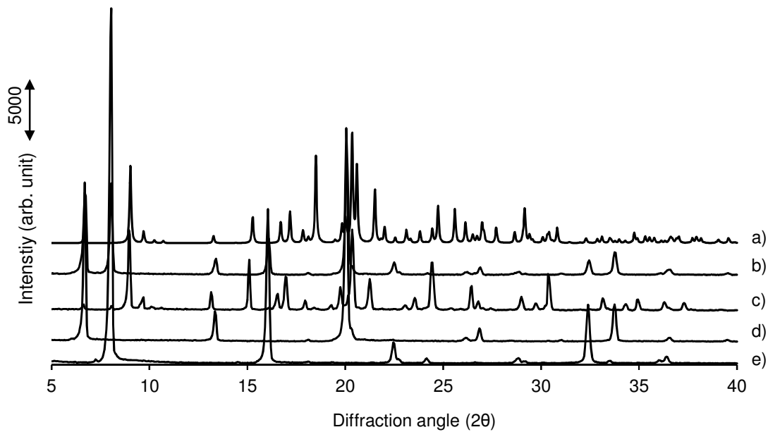
Figure 1: PXRD patterns of (a) 1:1 BA:DBSO cocrystal calculated based on single crystal data, (b) BA:DBSO (1:1) physical mixture, (c) 1:1 BA:DBSO cocrystal, (d) pure DBSO and (e) pure BA.
