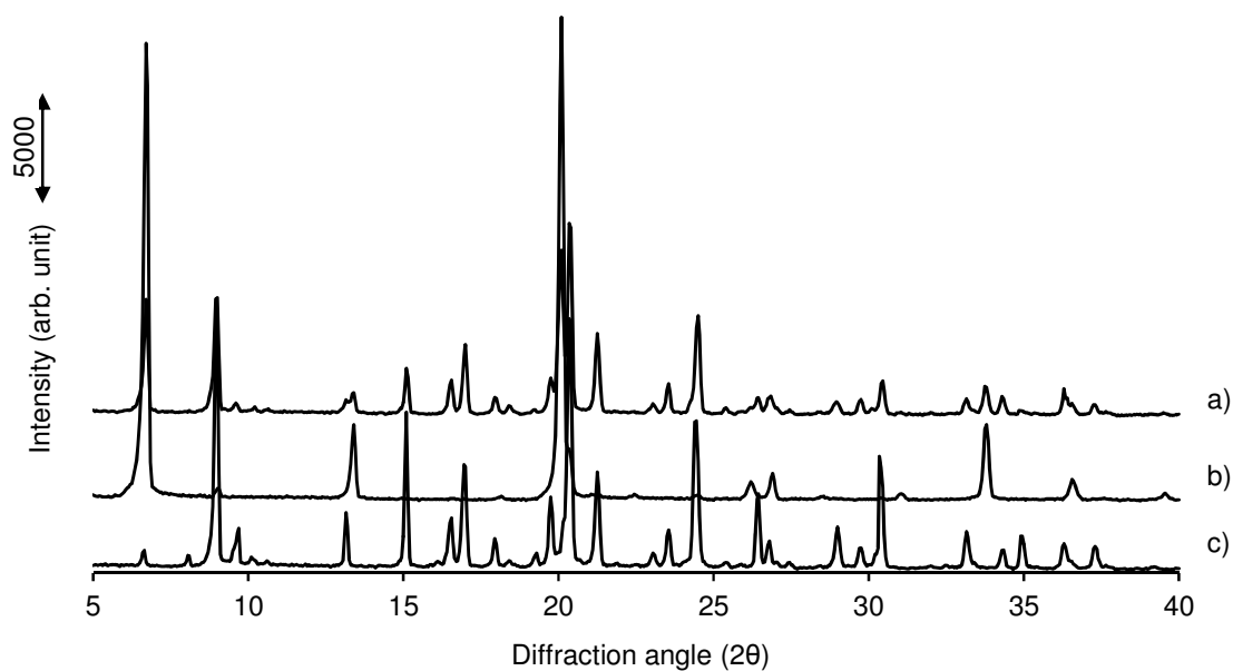
Figure 5: PXRD patterns of (a) remaining solid (12mg/mL BA added) after 24 hours solubility study, (b) remaining solid (12mg/mL BA added) after 12 hours solubility study, (c) 1:1 BA:DBSO cocrystal.
