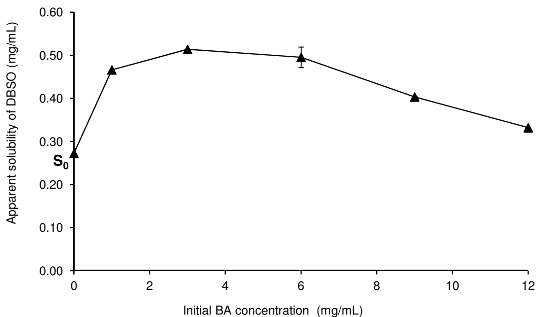
Figure 6: Solubility profile of DBSO after 24 hours where cocrystal is the excess phase in dependency of BA. S_0 represents the DBSO concentration in the absence of BA.
