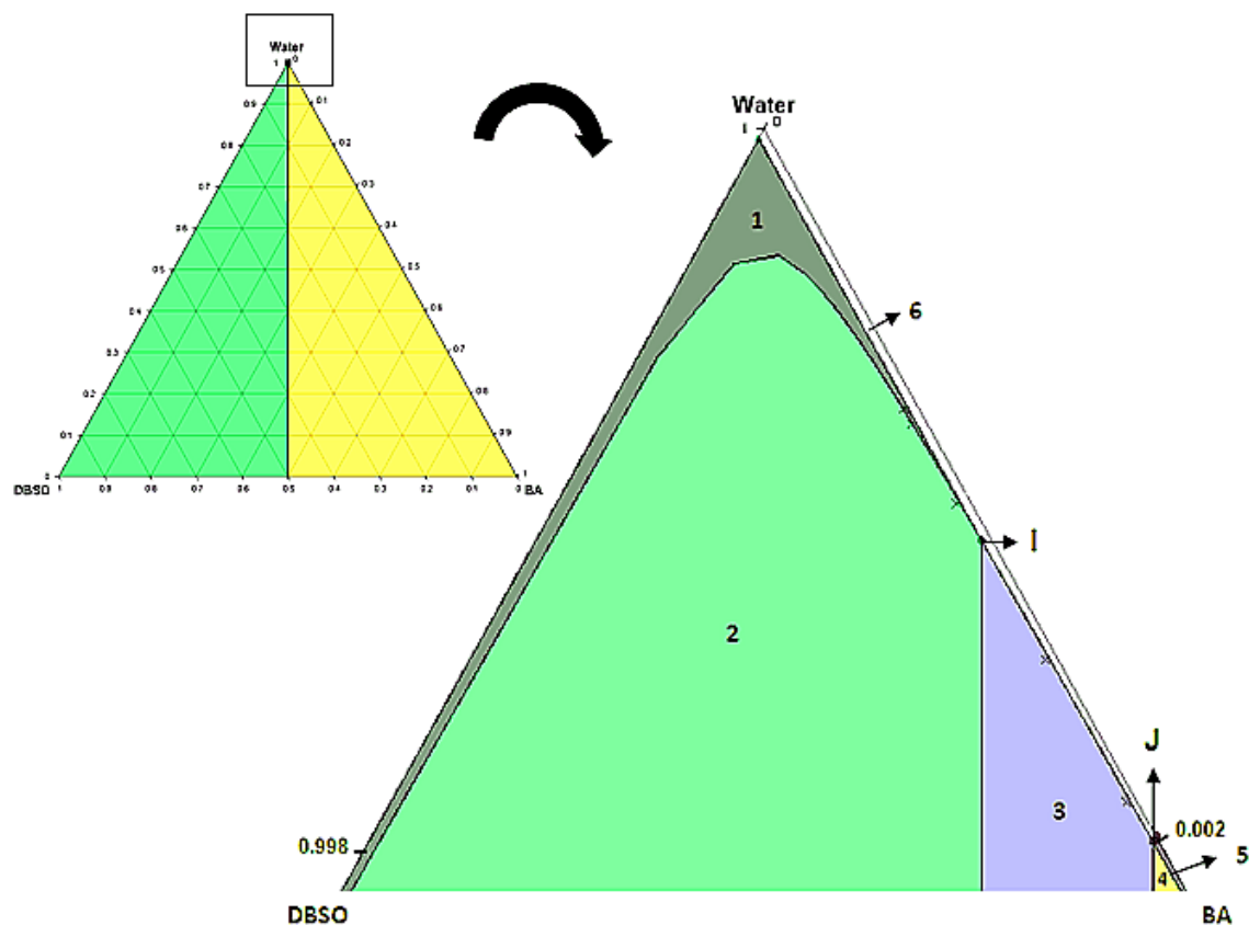
Figure 9: Zoom and downscaled view of ternary phase diagram of 1:1 BA:DBSO cocrystal in water at 37 °C (in mole fractions).
