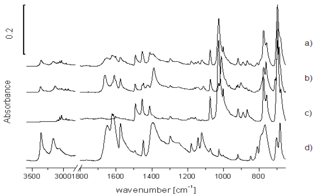
Figure 3: FTIR spectra of (a) BA:DBSO (1:1) physical mixture, (b) 1:1 BA:DBSO cocrystal, (c) pure DBSO and (d) pure BA.
