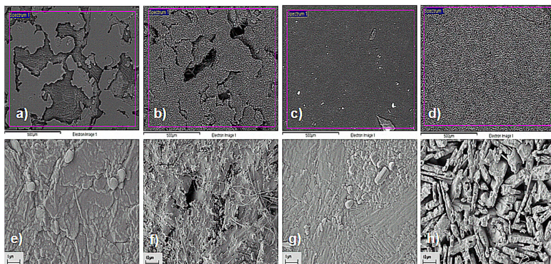
Figure 12: Backscattered electron images of solid compacts of (a) BA:DBSO (1:1) physical mixture before dissolution, (b) BA:DBSO (1:1) physical mixture after dissolution, (c) 1:1 BA:DBSO cocrystal before dissolution and (d) 1:1 BA:DBSO cocrystal after dissolution and secondary electron images of (e) BA:DBSO (1:1) physical mixture before dissolution, (f) BA:DBSO (1:1) physical mixture after dissolution, (g) 1:1 BA:DBSO cocrystal before dissolution and (h) 1:1 BA:DBSO cocrystal after dissolution.
