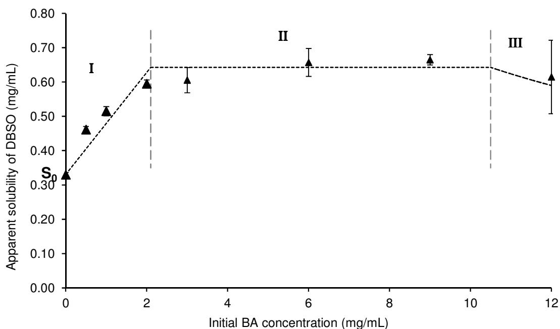
Figure 4: Profile of the apparent solubility of DBSO (mg/mL) as a function of BA concentration measured after 24 hours. S_0 is the DBSO concentration in absence of BA.
