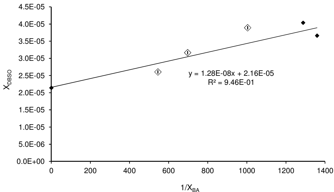
Figure 10: DBSO in equilibrium with cocystal (closed diamonds) as a function of the inverse total BA concentration at 37 °C (in molar fractions). Open diamonds represent solubility data beyond the equilibrium state. Trendline refers to closed diamonds.
