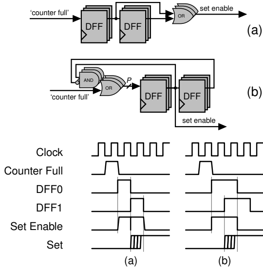
Fig. 2: Schematic and timing diagram of set enable logic: (a) simple circuit with potential glitch, (b) proposed glitch-free circuit.
