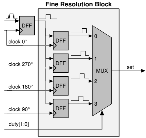
Fig. 4: Schematic of Fine Resolution Block.
