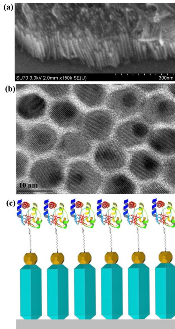
Fig. 1. Side view HRSEM image of (a) perpendicularly aligned nanorods (b) HRTEM top down image of gold tipped nanorods (c) schematic showing the bottom up assembly process consisting of gold tipped nanorods on an ITO substrate
