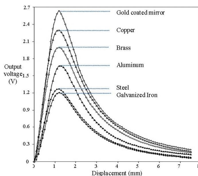
Figure 3. Response of fibre optic reflectivity of different reflector materials [31].
