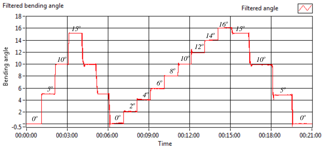
Figure 8. Bending measurement—bending angle (°).
