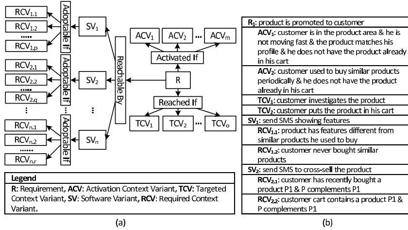
Fig. 1. The relation between Requirements, Context, and Software.
