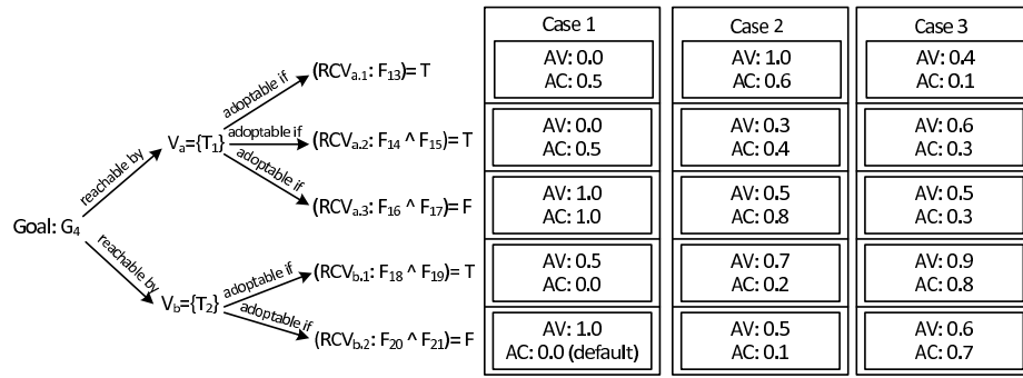
Fig. 3. Three different autonomic evolution scenarios involving the computation of AV and AC.
