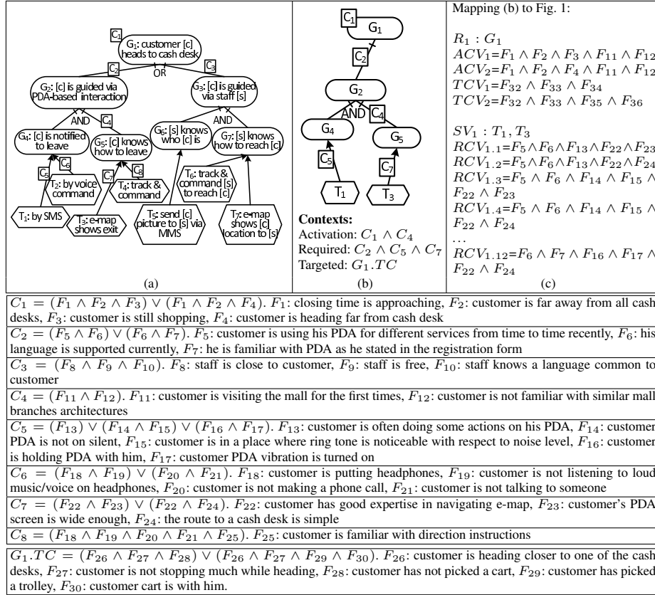
Fig. 2. An example of a Contextual Goal Model
