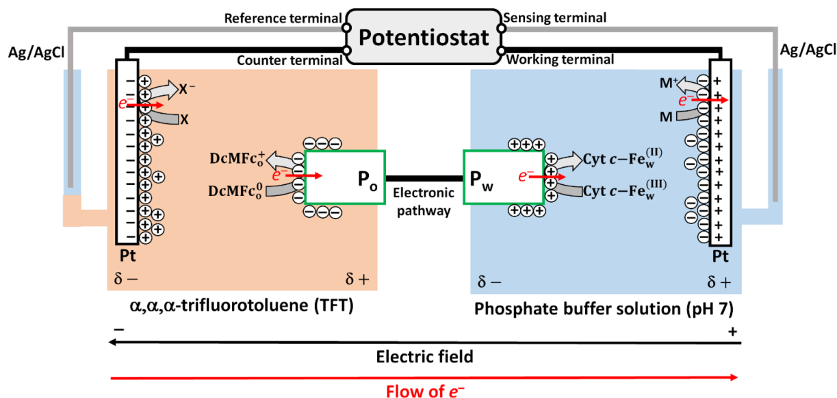
Scheme 2. Schematic of the 4-electrode CBPEC configuration with aqueous-organic electrolyte solutions used for the study of Cyt c bioelectrochemistry as \Delta\phi^w is biased sufficiently positively by the potentiostat to facilitate electron transfer along the BPE from the organic electron donor DcMFC at P_o to the aqueous Cyt c molecule at P_w .
