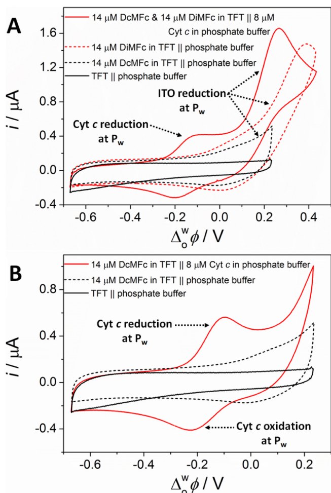
Fig. 1. (A) CVs obtained using the 4-electrode CBPEC configuration with aqueous-organic electrolyte solutions outlined in Scheme 1, in the absence of Cyt c and both ferrocene derivatives (solid black line), in the presence of 14 \mu\text{M} DcMFC only (dashed black line), in the presence of 14 \mu\text{M} DiMFC only (dashed red line), and in the presence of 8 \mu\text{M} Cyt c , 14 \mu\text{M} DiMFC and 14 \mu\text{M} DcMFC (solid red line). The scan rate used was 20 \text{mV}\cdot\text{s}^{-1} . (B) CVs obtained using the 4-electrode CBPEC configuration outlined in Scheme 1, as described in (A), using a smaller polarisable potential window to clearly observe the redox response at \Delta_0^w \phi_{1/2} = -0.161 V in the presence of 8 \mu\text{M} Cyt c and 14 \mu\text{M} DcMFC (solid red line). The scan rate used was 20 \text{mV}\cdot\text{s}^{-1} .
