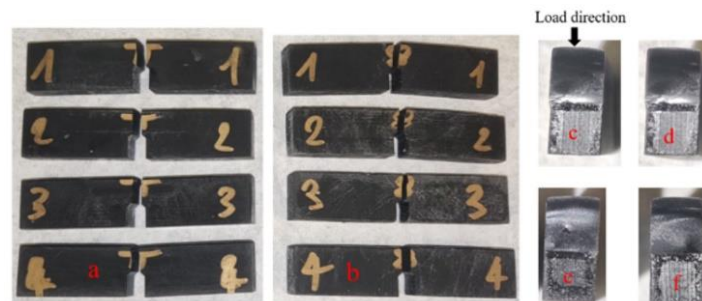
Figure 6. Failed SENB specimens (a) TGX, (b) TGX-UV, (c) TG0, (d) TGX, (e) TG0-UV and (f) TGX-UV
