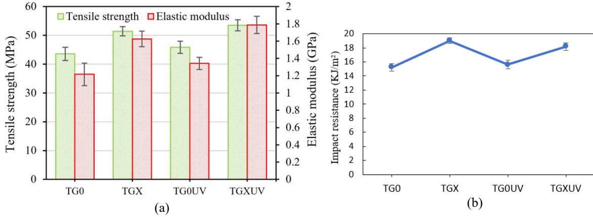
Figure 4. (a) Tensile strength and elastic modulus, and (b) impact resistance of the 3DPd specimens.
