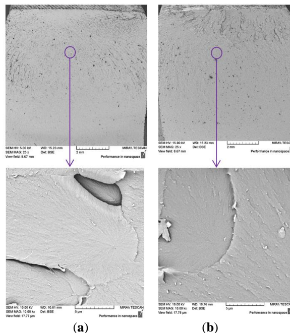
Figure 7. SEM of the (a) TG0 and (b) TGX of the failed SENB specimens
