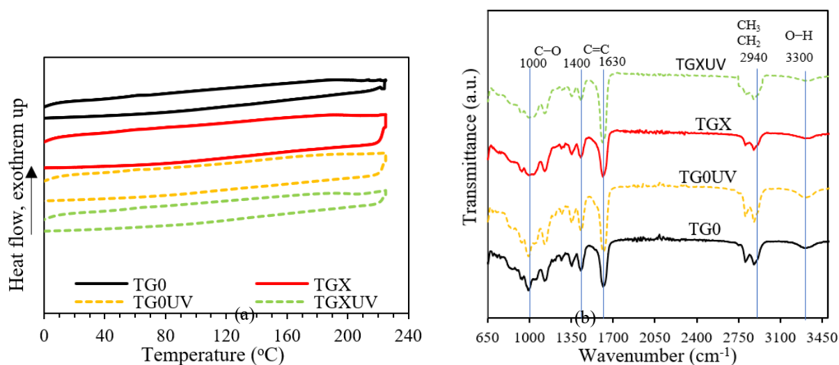
Figure 8. Thermal and chemical behaviour (a) DSC analysis and ; (b) FTIR spectra.
