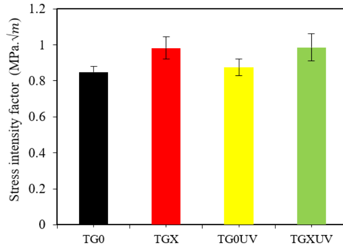
Figure 5. Stress intensity factor values of the SENB specimens
