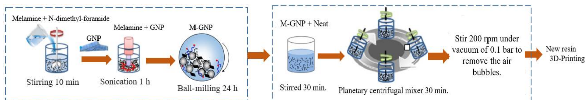
Figure 1. Schematic illustration of Ball-milling process to functionalise GNP by melamine.
