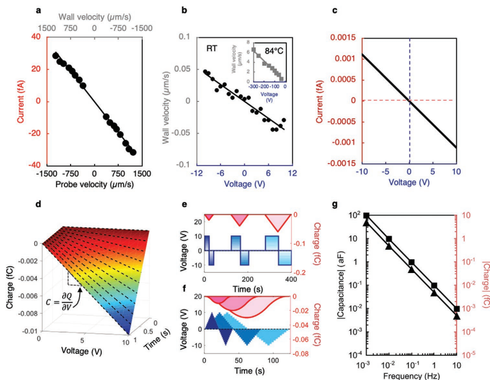
Figure 4. a) The CGM current under different scan-rates, measured either when moving toward (positive velocity) or away from (negative velocity) the 90^\circ in-plane head-to-head domain wall in the Cu–Cl boracite. b) The velocity associated with the anomalous field-driven motion of these head-to-head walls, as a function of switching bias applied to a positive surface electrode (the main panel data have been determined from in situ scanning probe microscopy at room temperature, while the inset shows data taken from in situ optical microscopy, performed at 84^\circ\text{C} , using geometries similar to those associated with Figure 2 and the Movies S2–S4, Supporting Information). c) By combining data from (a) and (b), the tip current (at a given velocity) can be expressed as a function of the switching voltage needed to induce the same relative motion between tip and domain wall. d) Given that the wall velocities are constant in time (for each driving voltage), the current–voltage relation given in (c) can be unpacked into a charge–time–voltage plot, allowing the capacitance to be explicitly determined, as a function of the time over which relative motion between electrode and wall occurs. e) Since the wall displacement is a linear function in time (the wall velocity is constant for each applied switching bias), the total charge collected at a sensing electrode can be calculated for different square pulse frequencies and hence modeled for more complex ac signals (such as the triangular pulses in (f)). g) The accumulated charge and hence negative capacitance can then be expressed as a function of ac signal frequency (squares indicate capacitance and charge from square waveforms and triangles from triangular waveforms). Note the gradient in the log–log plot shows that the magnitude of the negative capacitance is inversely related to frequency, passing Jonscher’s test for negative capacitance being inappropriately attributed to inductance.
