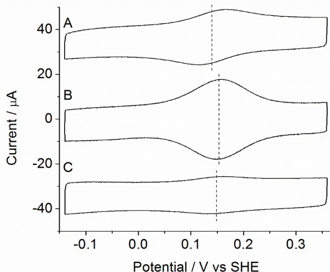
Fig. 5. Cyclic voltammograms of cyt c 550 (A), cyt c 550 [C] (B) and cyt c 550 [N] (C) immobilized on gold NPs modified with a 1/1 mixture of 6-mercaptohexan-1-ol and 1-hexanethiol (scan rate 0.1 V.s -1 , pH 7).
