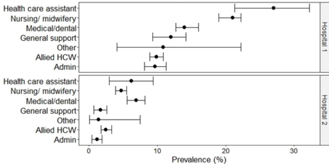
Figure 1: Proportion of staff group with detectable antibodies to SARS-CoV-2, both hospitals, October 2020*
