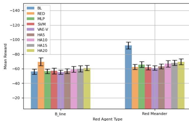
Figure 10. Performance comparison using Network Topology 2—100-step episode.
