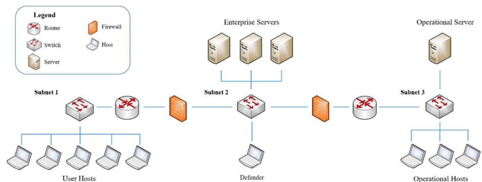
Figure 3. A networking scenario in CybORG [24].
