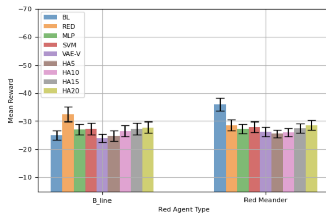
Figure 11. Performance comparison using Network Topology 2—50-step episode.
