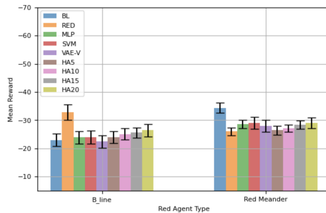
Figure 8. Performance comparison using training network topology—50-step episode.
