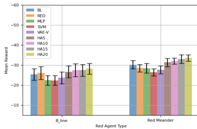
Figure 14. Performance comparison using Network Topology 3—50-step episode.
