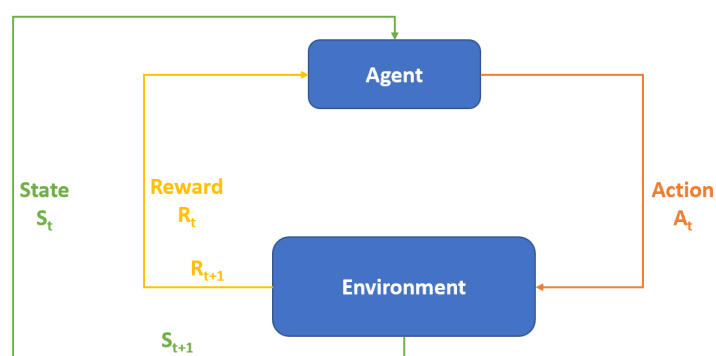
Figure 2. Reinforcement learning process.
