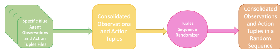
Figure 5. Preparing data for supervised learning.
