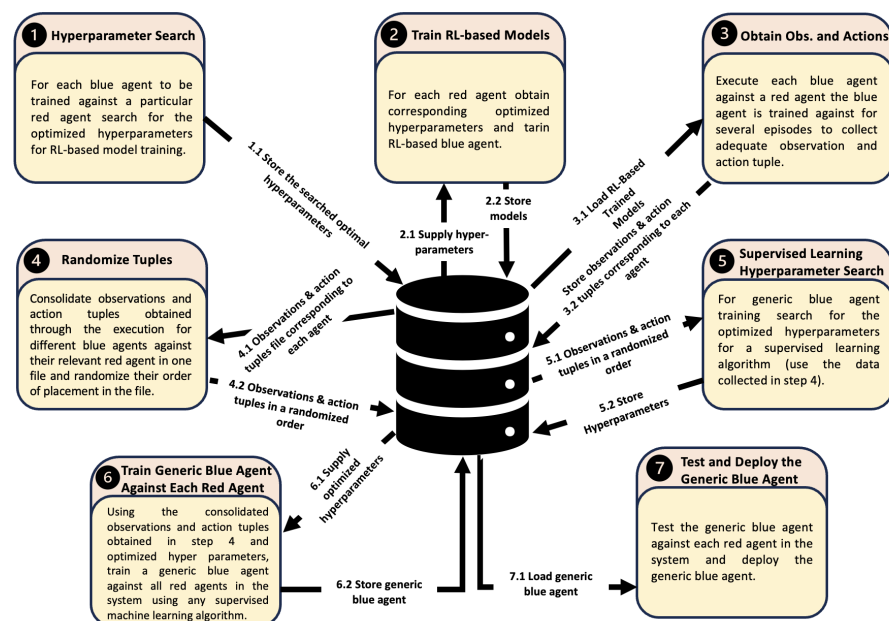
Figure 4. Proposed framework for generalized blue agent.
