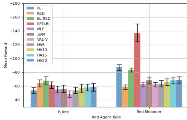
Figure 7. Performance comparison using training network topology—100-step episode.
