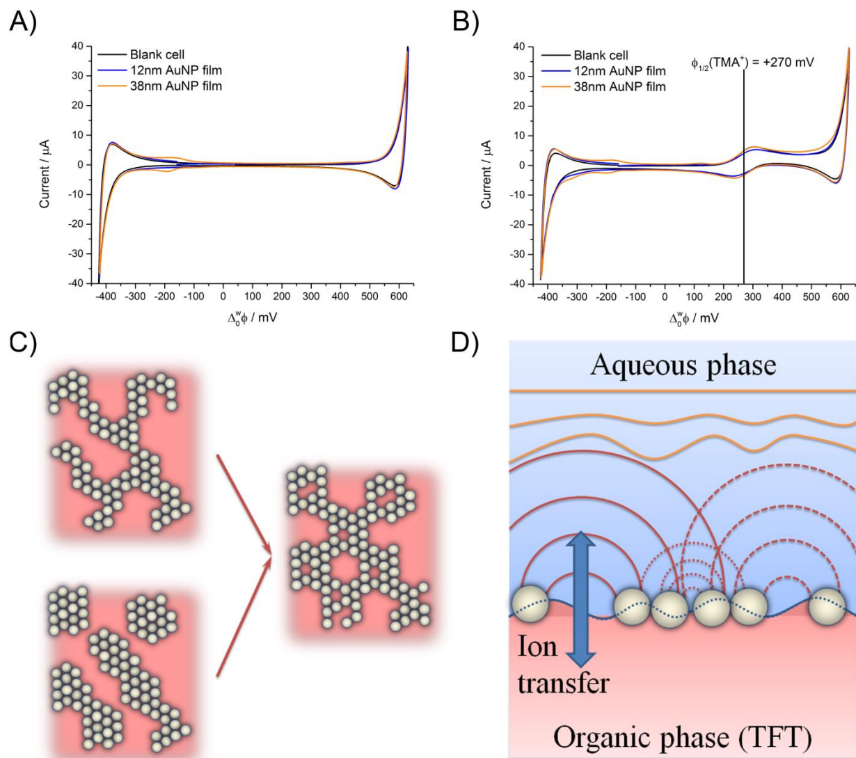
Figure 2. Cyclic voltammetry (CV; IR compensated) at bare and AuNP nanofilm modified soft interfaces formed between a 10 mM LiCl aqueous solution and a 5mM BATB solution in TFT. CVs were obtained at a scan rate of 25mV/s A) without, and B) with TMA + ions present for calibration. C) Schematic representation of possible distribution of AuNPs in the nanofilm at ITIES: randomly distributed network (top), islands with voids (bottom) and mixed morphology (middle). D) Schematic representation of the cross-sectional view of the ITIES partially occupied by a nanofilm of AuNPs (lines show the diffusion profiles of ion concentration).
