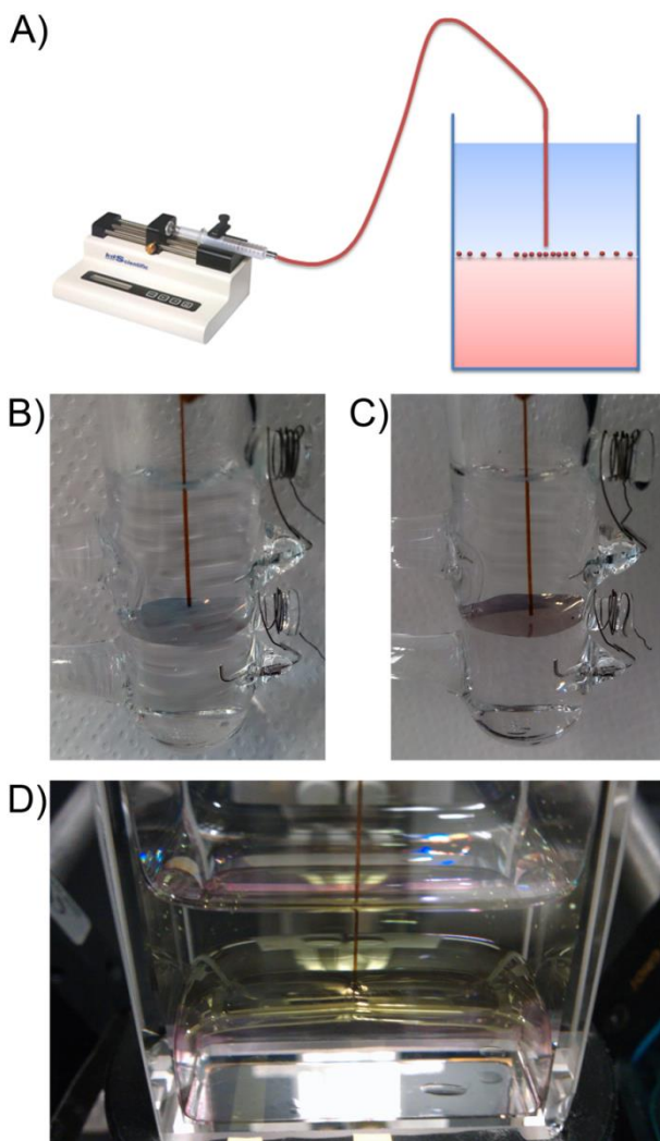
Figure 1. Functionalization of soft interfaces with AuNP nanofilms by precise injection of AuNPs suspended in methanol at the interface. (A) Schematic of the capillary and syringe-pump setup used to settle AuNPs directly at the interface between two immiscible liquids allowing precise control over the AuNP surface coverage. Examples of AuNP films prepared at flat soft water | trifluorotoluene interfaces in 4-electrode electrochemical cells using AuNPs with mean diameters of (B) 12 nm and (C) 38 nm. Flat soft interfaces were achieved by partial silanization of the bottom
