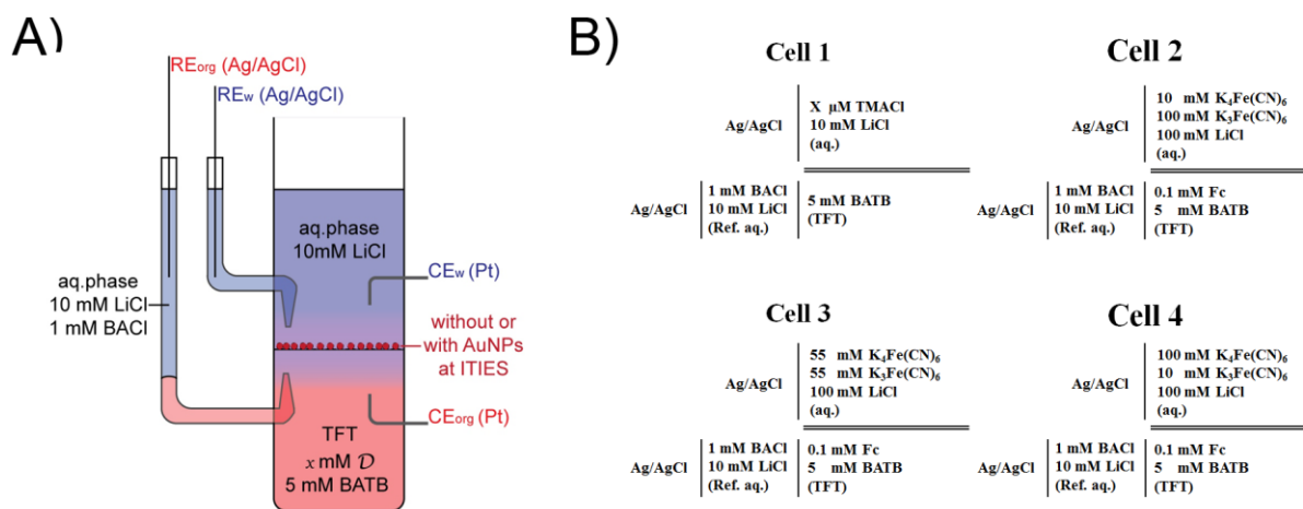
Scheme 4. A) Scheme of the four electrode electrochemical cell and B) composition of the four-electrode electrochemical cells utilized in this study. \mathcal{D} denotes electron-donor molecules such as Fc.
