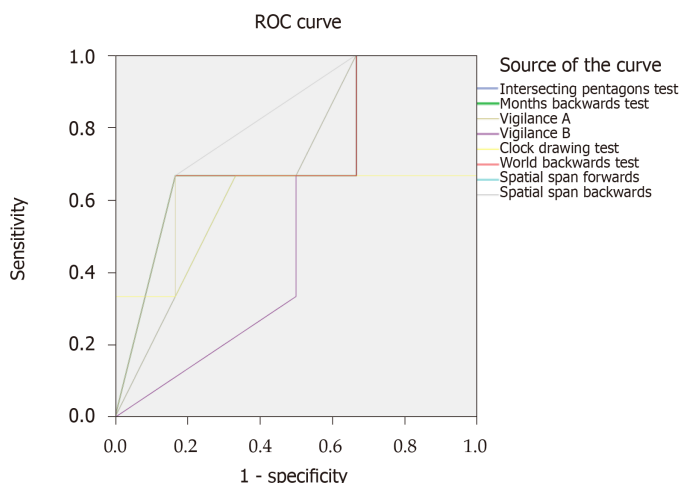
Figure 3 Receiver operating characteristic analyses depicting the accuracy of conventional bedside tests of cognition for delirium diagnosis in the overall population (n = 180). ROC: Receiver operating characteristic analyses.
